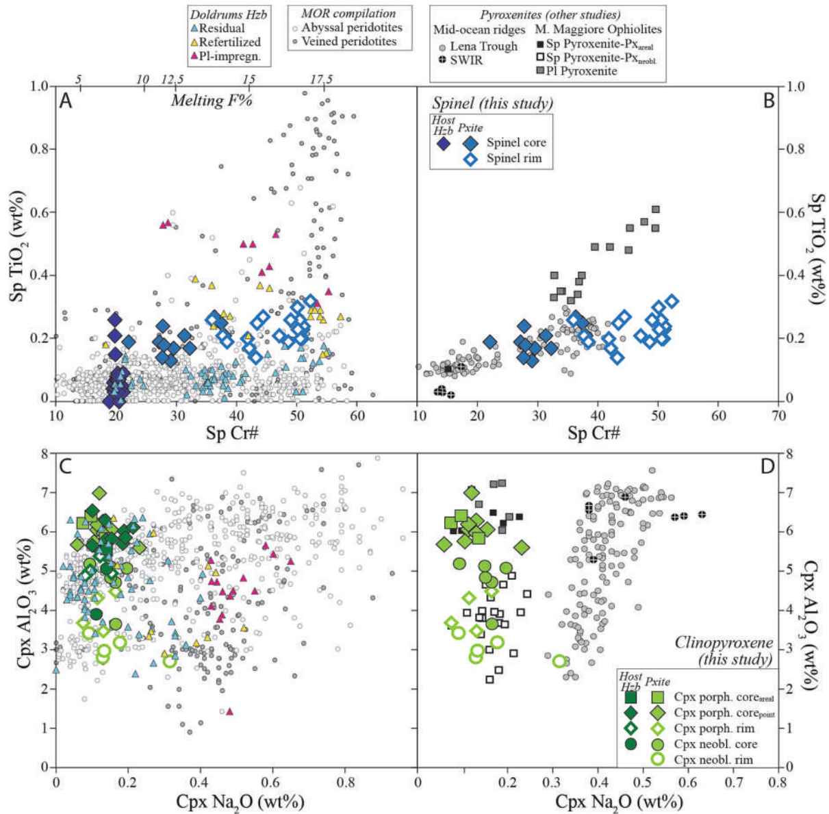
Fig. 4. Spinel (A–B) and clinopyroxene (C–D) major element compositions from the pyroxenite vein (Pxite) and its host harzburgite (Host Hzb). (A–B) Cr# [Cr# = 100 × cationic molar (Cr/(Cr + Al))] values versus TiO 2 contents in spinel; analyses at crystal rims were performed in the pyroxenite only. The degree of mantle melting (F%) in (A) is based on the spinel Cr# following Hellebrand et al. (2002). (C–D) Na 2 O versus Al 2 O 3 contents in clinopyroxene porphyroclasts and neoblasts. In (A) and (C) we report all data from this study in comparison with residual, refertilized and PL-impregnated peridotites from the Doldrums FZ (Sani et al., 2020) and abyssal mantle peridotites from mid-ocean ridges (abyssal and veined peridotites from Warren, 2016). In (B) and (D) the compositions of pyroxenites are plotted including those from other spreading centers (Lena Trough, Laukert et al., 2014; SWIR, Dantas et al., 2007) and ophiolitic analogues (Monte Maggiore Ophiolite, Corsica, Basch et al., 2019).
