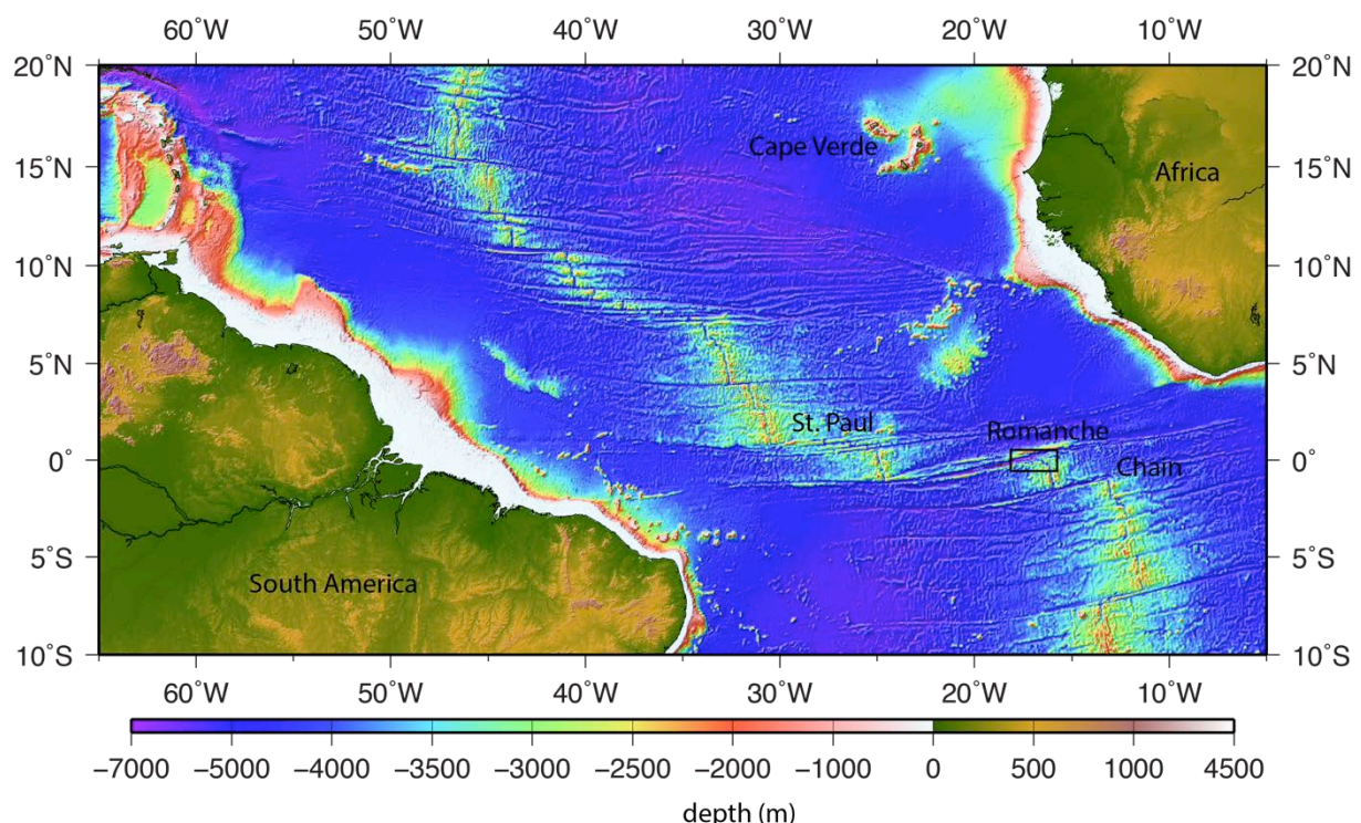
Figure 1. General bathymetry (from satellite data) of the Equatorial Atlantic. The SMARTIES area corresponds to the rectangle.
