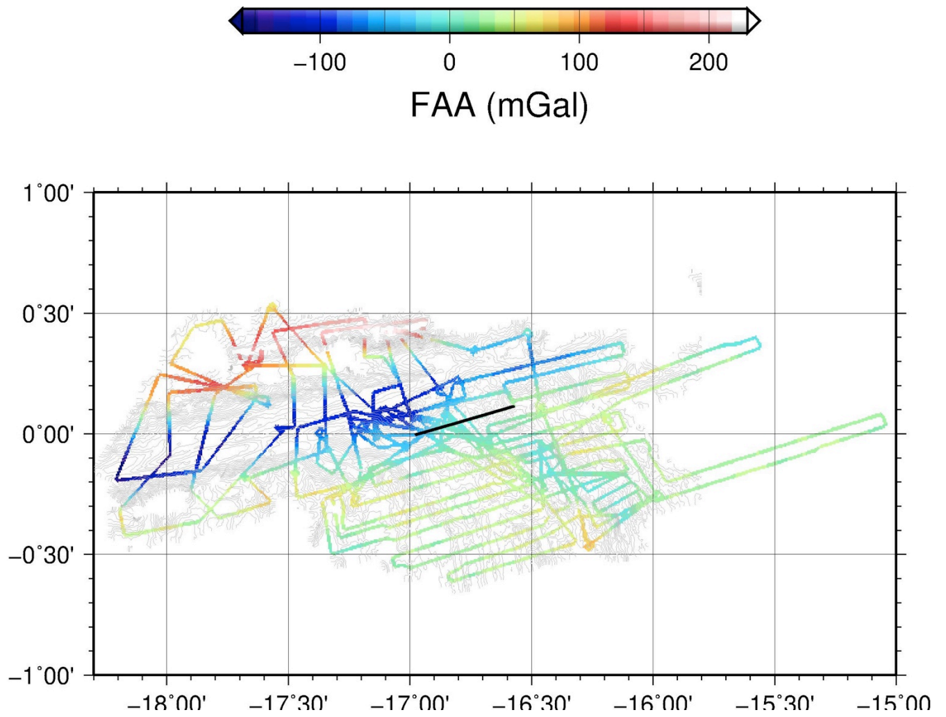
Figure 5. Preliminary gravity results along the 172 SMARTIES gravimetric profiles. The solid black line shows the location of the profile n. 22, whereas the thin grey contours are the newly acquired high-resolution bathymetry (300 m spacing). Colored grid spacing corresponds to 300 m, with interpolation search radius equal to 1 km.
