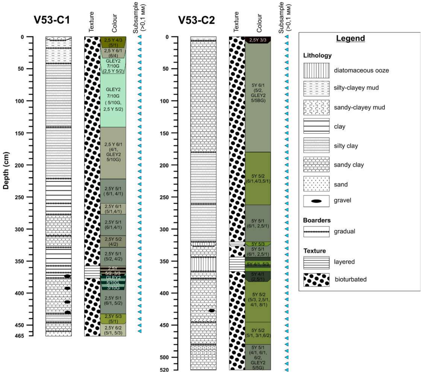
Fig. 15 - Lithological description of the sedimentary gravity cores V53-C1 and V53-C2 recovered at the Charlie Gibbs FZ. Detail of the texture, colour and location of subsampling is represented in the right column for both cores.
