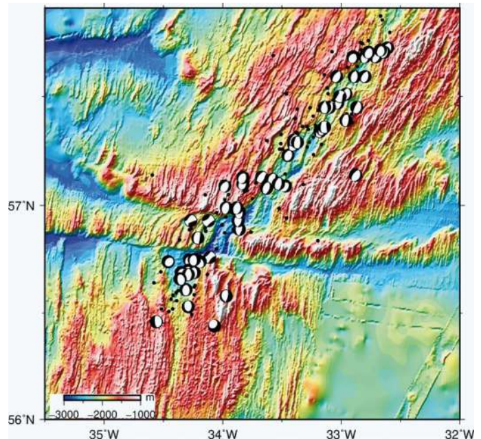
Fig. 4 - Seismicity of the Bight transform region from the International Seismological Centre Event catalogue ( www.isc.ac.uk ). Focal mechanisms (beach balls) are from the Centroid Moment Tensor (CMT) catalogue ( www.globalcmt.org ). Fault plane solutions show prevalent E-W extension along the northern Mid Atlantic Ridge segments, with centroid depths ranging from 5 to 19 km.
