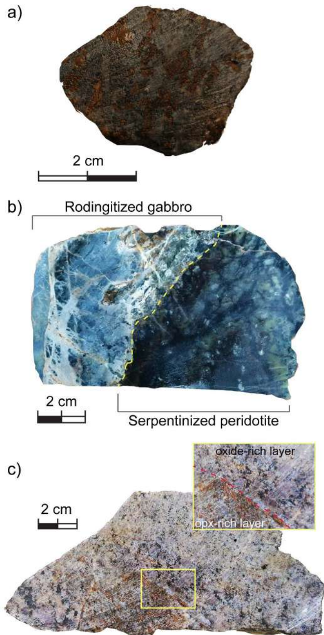
Fig. 12 - Hand-sample photographs of the recovered gabbroic rocks; a) Sub-ophitic gabbro recovered from OCC structures in the Charlie Gibbs ITR Domain; b) Rodingitized gabbro in contact with a serpentinized peridotite sampled from the northern transform wall of the Charlie Gibbs northern transform valley; c) Gabbroic sample showing a diffuse contact between an oxide gabbro layer and a gabbro-noritic layer, recovered from an off-axis bathymetric high east from the MAR axis, south of the Bight FZ.
